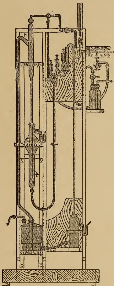
Fig. 91. AUTOMATIC LOW-PRESSURE AIR PUMP FOR THE DISTILLATION OF UNSTABLE SUBSTANCES IN THE HYDRO-CARBONS.
